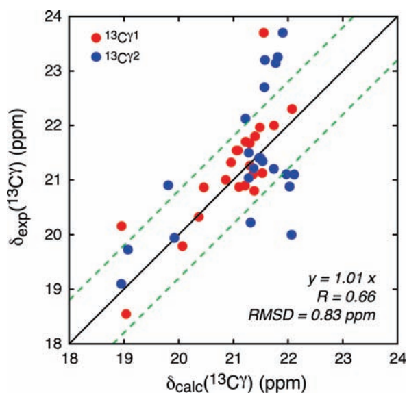
Figure 2. Comparison of experimentally measured ^{13}\text{C}^\gamma chemical shifts, \delta_{\text{exp}} , with chemical shifts derived from the J -reference ensemble and calculated using a DFT-derived hyper-surface (Figure 1b) and eq 3, \delta_{\text{calc}} . ^{13}\text{C}^{\gamma 1} , ^{13}\text{C}^{\gamma 2} , ^{13}\text{C}^{\gamma 1} , ^{13}\text{C}^{\gamma 2} , ^{13}\text{C}^{\gamma 1} , ^{13}\text{C}^{\gamma 2} chemical shifts are shown in red (blue); green dotted lines are given by y = x \pm \sigma , where \sigma = \text{rmsd}(\delta_{\text{calc}} - \delta_{\text{exp}}) .
