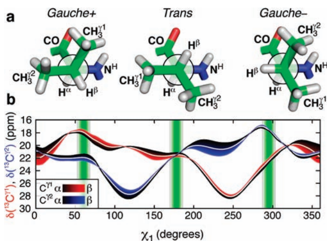
Figure 1. (a) Three canonical rotamer conformations of the Val side-chain based on a database of high-resolution crystal structures. 30,31 (b) 13 C γ1 (red; pro-R ) and 13 C γ2 (blue; pro-S ) chemical shifts derived from a DFT calculation for \beta -sheet (light) and \alpha -helical (dark) backbone conformations (see Supporting Information for details); the average is shown with the white line. The green bars indicate the ‘canonical values’ from the set of high-resolution crystal structures, see text ( \chi_1 = 63^\circ \pm 9^\circ for gauche+; \chi_1 = 174^\circ \pm 9^\circ for trans; \chi_1 = 296^\circ \pm 9^\circ for gauche-).
