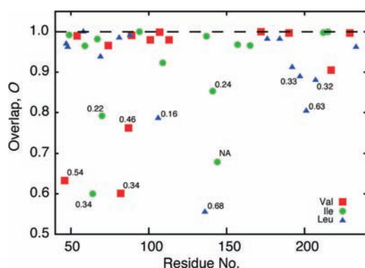
Figure 6. Plot of O values (eq 5) as a function of residue number for Ile, Leu, and Val residues of \alpha_7\text{-}\alpha_7 . Values of S_{\text{axis}}^2 , averaged over the \gamma_1 and \gamma_2 positions, are listed for residues where O values are \leq 0.9 .
