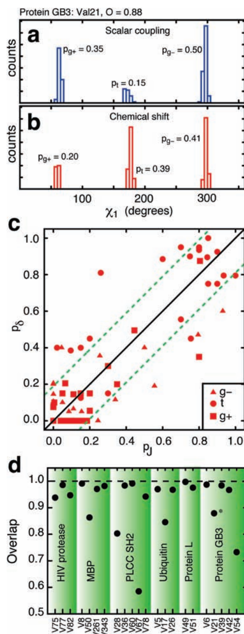
Figure 3. Comparison of rotamer ( g+ , t , g- ) populations determined from Val methyl-backbone three-bond scalar couplings and from chemical shifts, \delta(^{13}\text{C}^{\gamma 1}) and \delta(^{13}\text{C}^{\gamma 2}) . (a,b) Distributions calculated for Val 21 of protein GB3, based on input scalar couplings (a) or chemical shifts (b). The overlap, O , between the two distributions is calculated using eq 5. (c) Correlation plot of rotamer populations derived from chemical shifts ( p_\delta ) vs the corresponding values generated using scalar couplings ( p_\gamma ), as described in the text. (d) The overlap, eq 5, calculated for all the Val residues used in the simulations described above. Val 21 of protein GB3, that is ‘featured’ in a,b is marked with an asterisk.
